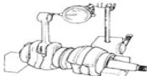
Fig. SZ11-13—Move connecting rod small end side to side to determine connecting rod, bearing and crank pin wear. Refer to text.
