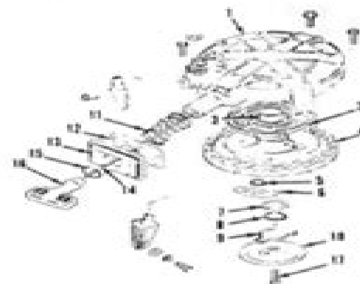
Fig. SZ11-15—Exploded view of manual starter assembly.
